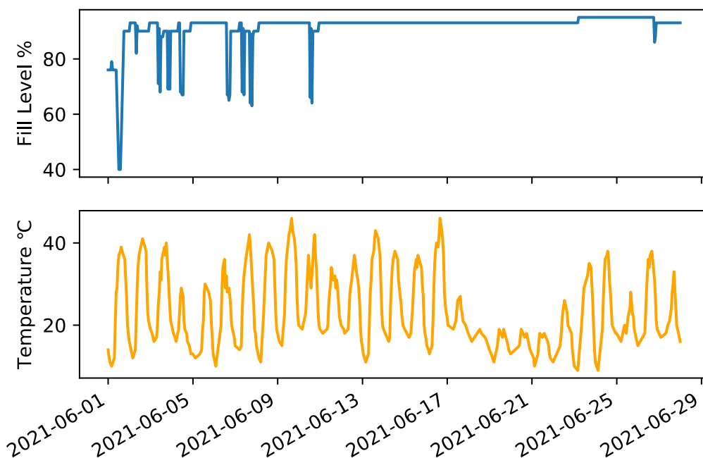
Figure 5: Fill level and temperature for sensor in grit bin at Adastral Park, during June 2021.
