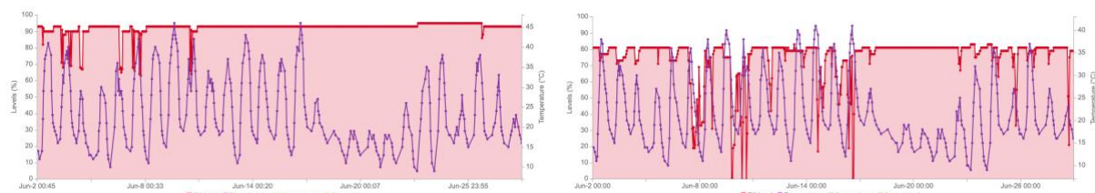
Figure 6: Fill level and temperature for sensors in grit bins, during June 2021, screengrabs from NetBin Hub, Left hand figure for sensor at Adastral Park, right hand figure for sensor at Melton.
