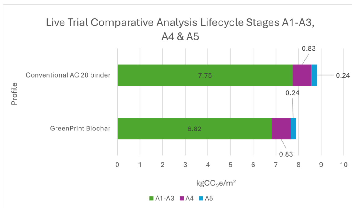
Figure 7: Comparative carbon analysis GreenPrint Biochar versus conventional AC20 A1-A3, A4 & A5 lifecycle stages per m 2
