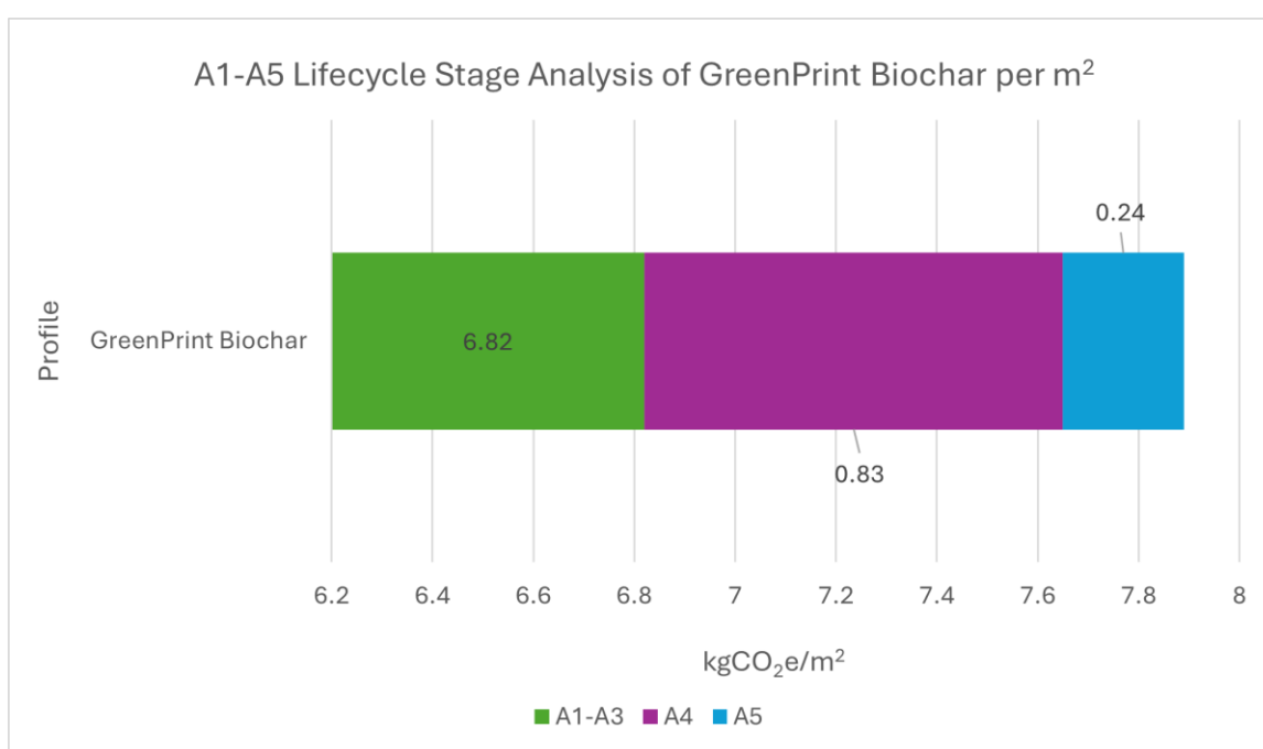
Figure 5: Carbon analysis of GreenPrint Biochar (1% Biochar) lifecycle stages A1-A3, A4 & A5 per m 2
